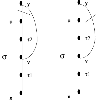
Figure 8: a) positive path preempts negative path b) negative path preempts positive path
