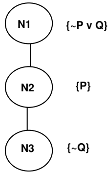
Figure 6: Doing a simple downward traversal will give the wrong answer for wff-inheritance
