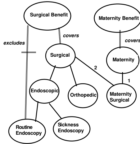
Figure 1: One method of representing coverage information: covers and excludes links are added to the standard subtype and cancels links of inheritance networks. Solid lines represent is-a links; slashed solid lines (not present here) represent cancels links; double lines represent covers links; slashed double lines represent excludes links. This representation can be mapped to a standard inheritance network.
