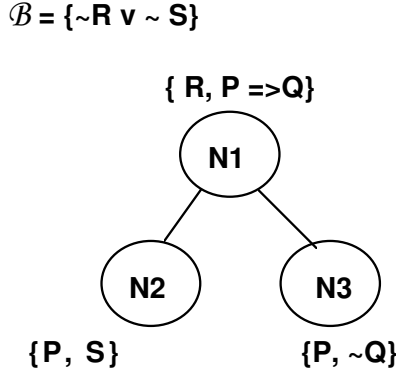
Figure 4: Taking the union of wffs at nodes yields inconsistency.
