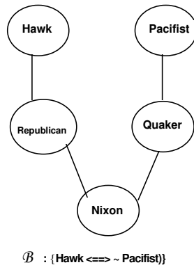
Figure 9: The modified Nixon diamond is inconsistent, but only implicitly.
