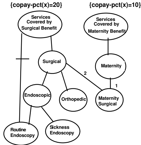
Figure 2: Representing coverage information in a standard nonmonotonic inheritance network. Lines represent is-a links; slashed lines represent cancels links. Medical benefits are reified as services covered by a particular benefit.
